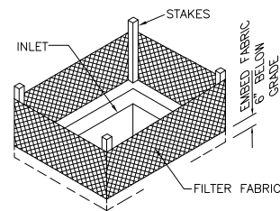
TEMPORARY FILTER FABRIC INLET PROTECTION DETAIL
