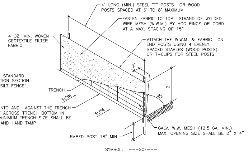
TEMPORARY SEDIMENT CONTROL FENCE DETAIL
