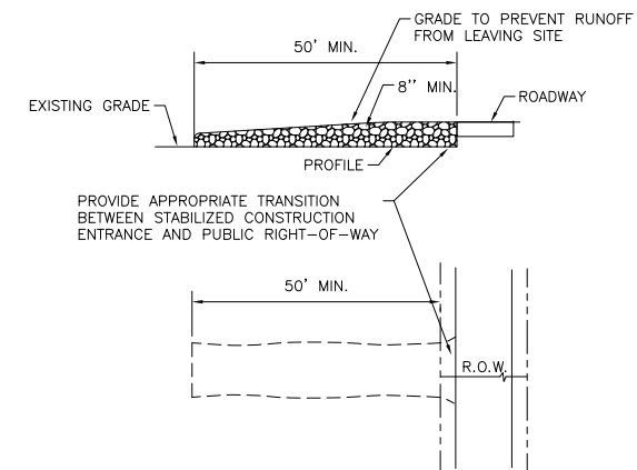
PLAN STABILIZED CONSTRUCTION ENTRANCE
