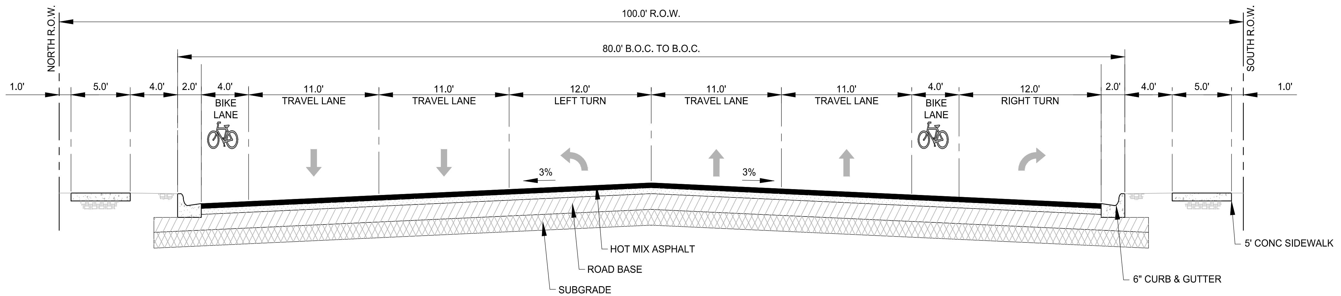
PROPOSED ROADWAY (STA. 19+34 THRU STA. 27+50)
