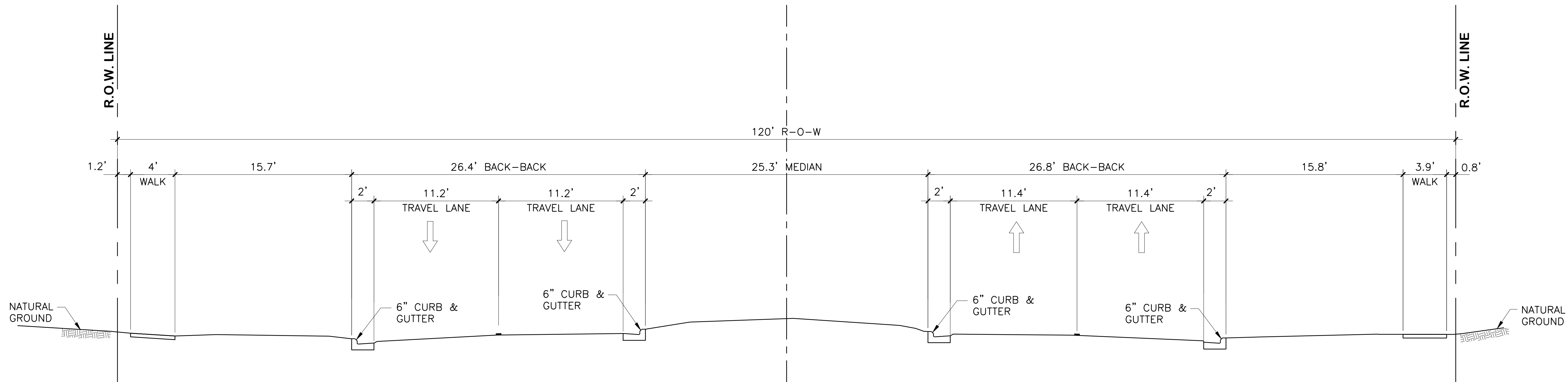
1 EXISTING ROADWAY SECTION SCALE = 1" = 5'
