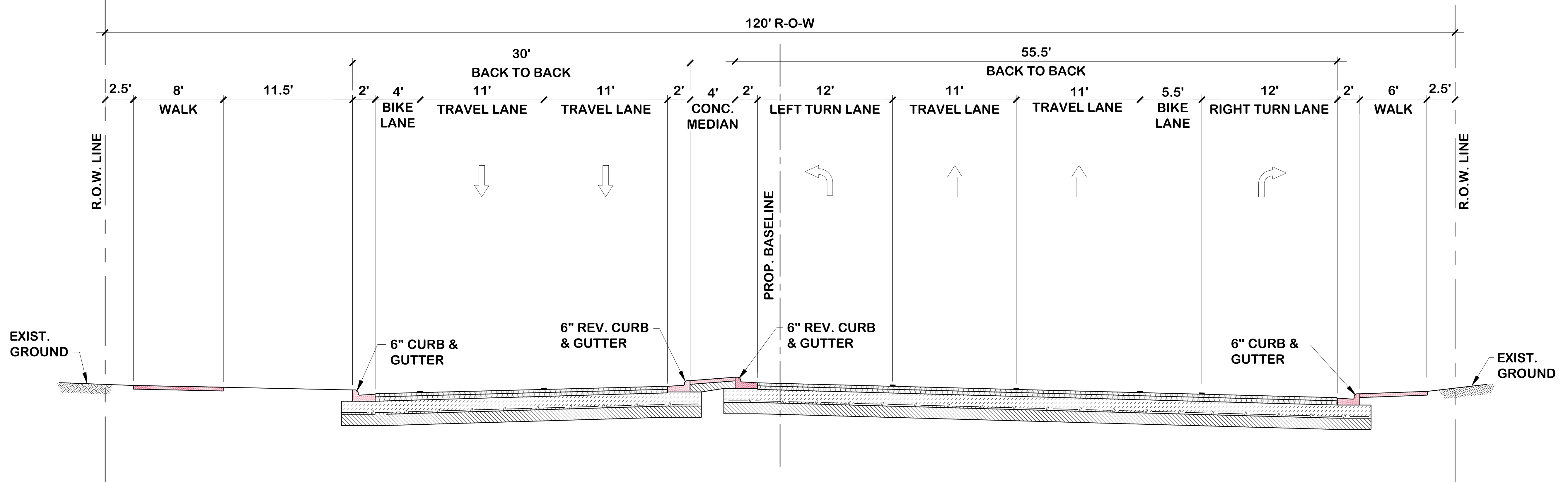
2 PROPOSED ROADWAY SECTION SCALE = 1" = 5'
